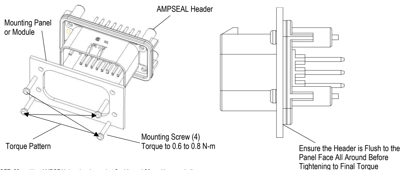
Figure 15 Panel Mounting Instructions
