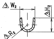
SEC. B-B
