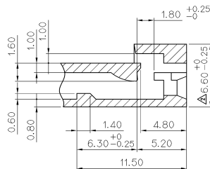
SECTION A-A (S=5/1)
