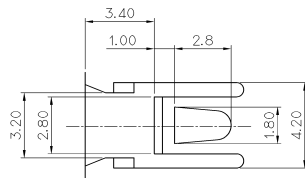
TERMINAL LOCK DETAIL
