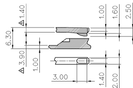
TERMINAL LOCK DETAIL (X2)
