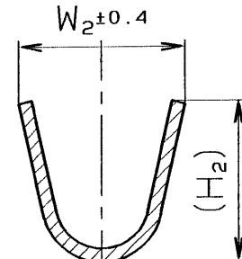
SEC. B-B
