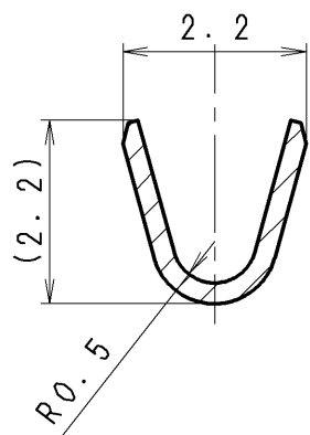
SEC. B-B
