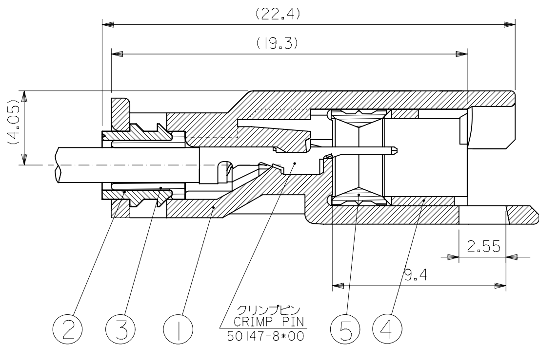
断面A-A (端子装着状態図) SECT.A-A(TERM.ASSEMBLY DRAWING)
