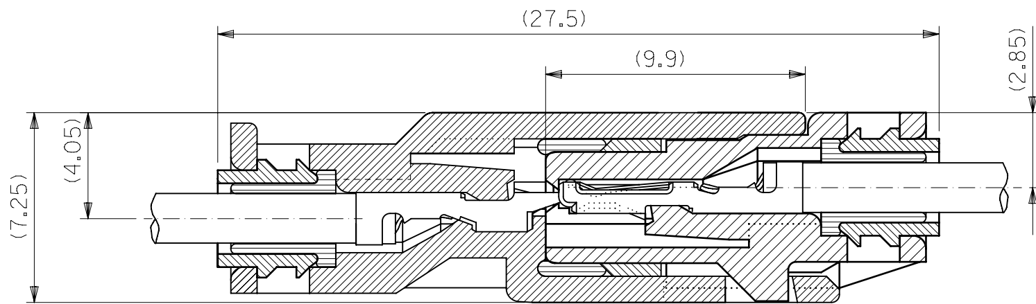
嵌合状態図 FULLY MATED CONDITION
